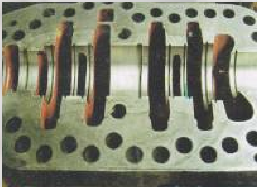
PUMP CASING
